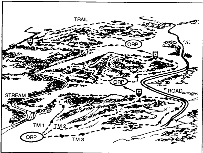
Figure 3-4. Box method.
